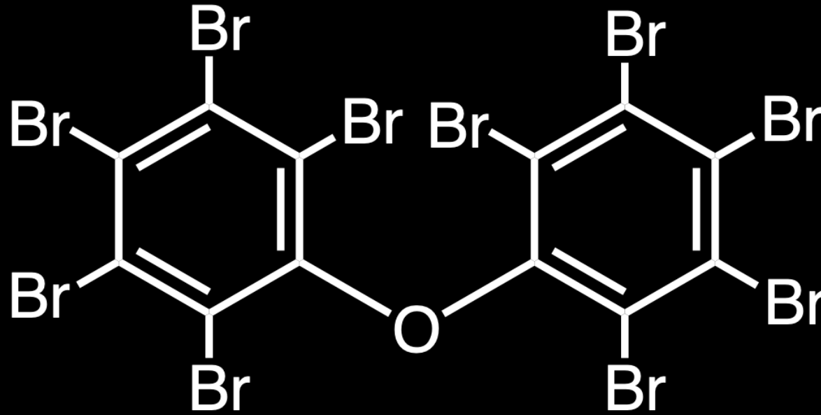
Decabromodiphenyl ether
