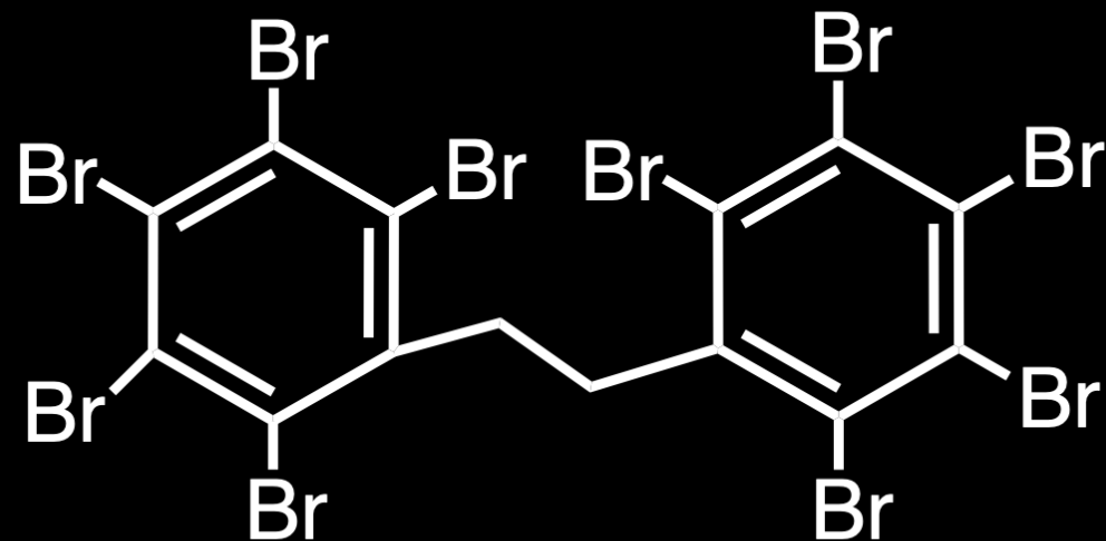
Decabromodiphenyl ethane
