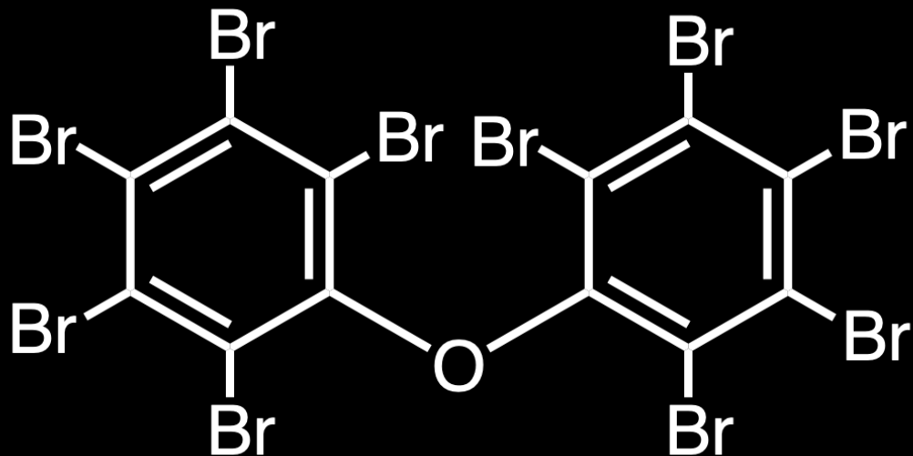
Decabromodiphenyl ether
