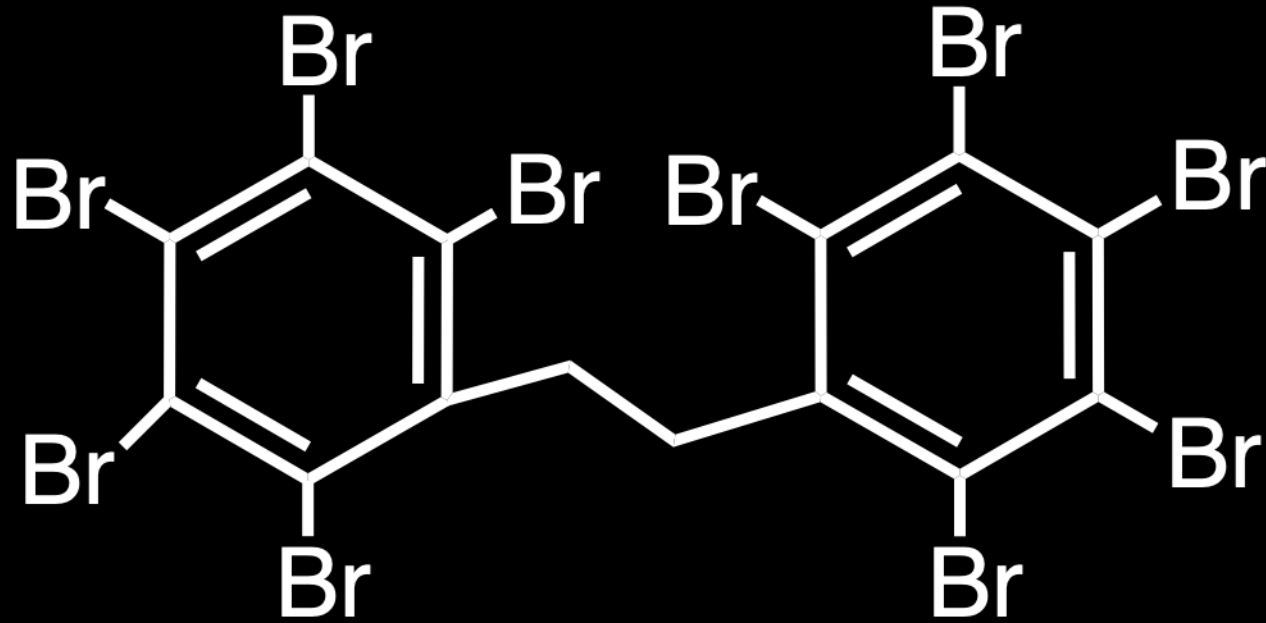
Decabromodiphenyl ethane
